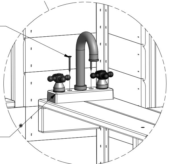
SCREW PFH 8x1 1/2 (2 PLCS)
