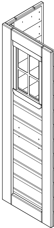
(1) WP1 - LEFT FRONT CORNER PANEL - W2A01524
