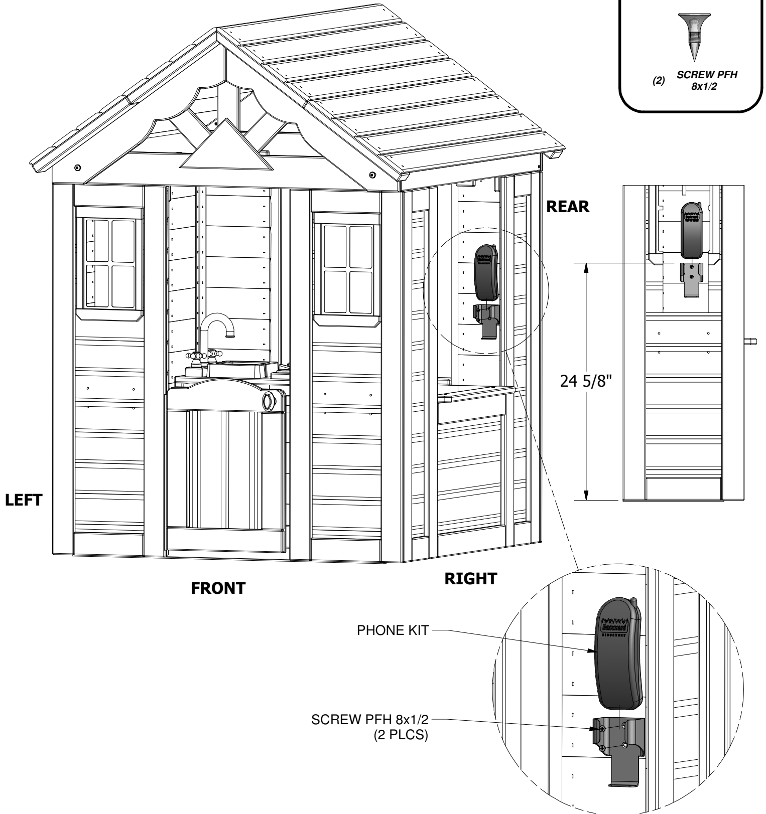
(1) PHONE KIT - A100132
